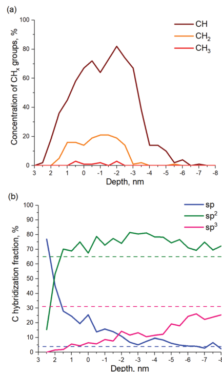
Fig. 10 (a) Relative concentration of \text{CH}_x groups in the H-modified a-C and (b) calculated profiles of carbon hybridization in the H-modified a-C layer. The initial values of \text{sp} , \text{sp}^2 and \text{sp}^3 hybridization are shown by dashed lines of the corresponding color.
