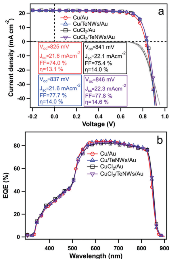
Fig. 5 (a) J - V characteristics and (b) external quantum efficiency (EQE) of CdTe solar cells with Cu/Au, Cu/TeNWs/Au, \text{CuCl}_2/\text{Au} and \text{CuCl}_2/\text{TeNWs}/\text{Au} back contacts respectively. The solid and dotted lines in Fig. 5(a) represent J - V curves under illumination and dark conditions respectively.
