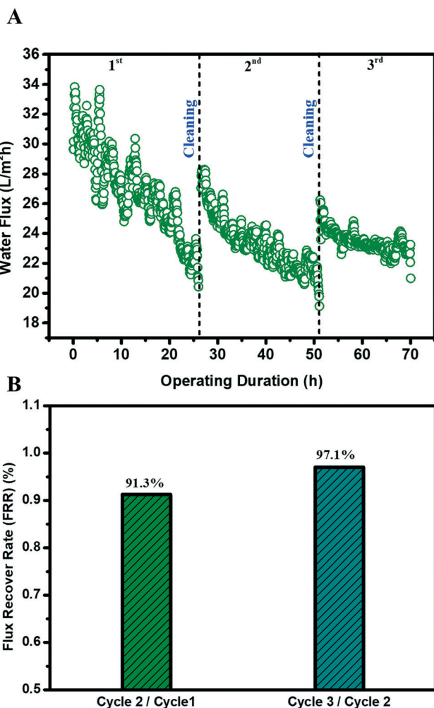
Fig. 6 Performance of the FTES modified membrane in membrane distillation after three fouling-cleaning cycles: (A) water flux decline curve; (B) calculated water flux recovery rate after each cycle. The water flux recovery was calculated as the ratio between the initial water fluxes of two consecutive filtration cycles.
