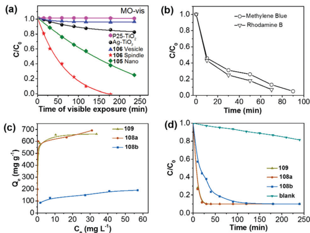
Fig. 22 (a) Comparative photocatalytic degradation of MO of commercial \text{TiO}_2 , \text{Ag-TiO}_2 , polymer nanofibers of 105 , vesicles and nanospindles of polymer 106 under visible light (P25- \text{TiO}_2 is \text{TiO}_2 with a diameter of 25 nm). (b) Photocatalytic degradation of RhB and MB using polymer 107 . (c) The adsorption isotherms of RhB for polymers 108a , 108b and 109 at 25 °C. (d) Removal of RhB with polymers 108a , 108b and 109 in the supernatant. Reprinted with permission from ref. 215–217. Copyright 2015 Nature Publishing Group, 2015 Wiley-VCH and 2015 Royal Society of Chemistry.
