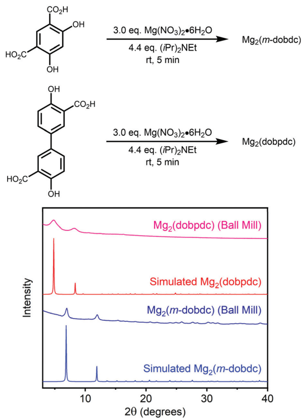
Fig. 6 Powder X-ray diffraction patterns ( \lambda = 1.5406 \text{ \AA} ) of Mg_2(m\text{-dobdc}) (blue) and Mg_2(dobpdc) (red) prepared under mechanochemical conditions. The simulated patterns based on the previously reported single-crystal X-ray diffraction structures of the isostructural frameworks Co_2(m\text{-dobdc}) 54 and Zn_2(dobpdc) 56 are included for reference.
