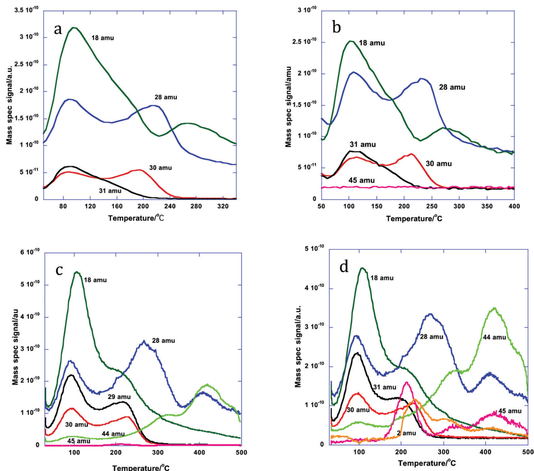
Fig. 3 Desorption products during TPD from the doped HSA Fe 2 O 3 samples, coated with 3 ML equivalent of MoO x : (a) 5% Al doped, (b) 10%, (c) 15% and (d) 20%.
