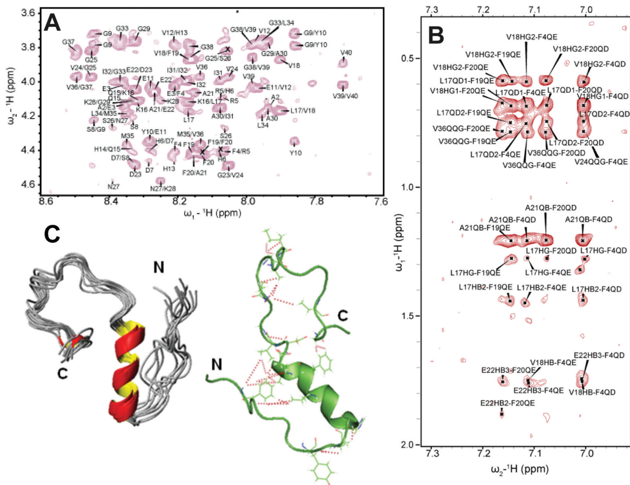
Fig. 5 3D structure of a small molecular weight A \beta_{1-40} intermediate determined by solution NMR. (A) 2D NOESY spectrum of 77 \mu\text{M} A \beta_{1-40} dissolved in 20 mM potassium phosphate, 50 mM NaCl, pH 7.3 containing 93% H _2 O and 7% D _2 O recorded at 15 ^{\circ}\text{C} on a 900 MHz NMR spectrometer. The selected regions show NOEs that corresponds to the sequential assignment of H _{\alpha i} –N _{H i+1} . (B) The aromatic region of the NOESY spectrum showing cross-peaks between F19 and F20 residues, the C-terminus and F4 residue, and the central helical region of the peptide. (C) 3D NMR structures of A \beta_{1-40} calculated from NOEs and backbone dihedral angle restraints. The cartoon structure shown on the right in green shows the long-range NOEs that stabilizes the formation of the hairpin structure and the bends in the N- and C-termini (red dashed lines). Copyright © 2011 Elsevier Inc. This figure is reproduced with permission from Biochemical and Biophysical Research Communications: DOI: 10.1016/j.bbrc.2011.06.133. Further details can be found in the published article. 69
