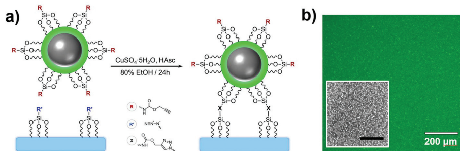
Fig. 10 (a) Grafting scheme of \text{Ag}@\text{(FL)} NPs to a \text{SiO}_2 substrate through \text{Cu}^I -catalyzed 1,3-dipolar cycloaddition. (b) Fluorescence image of the substrate grafted with \text{Ag}@\text{(FL)} NPs ( \lambda_{\text{exc}} = 489 \pm 6 \text{ nm} , \lambda_{\text{em}} = 536 \pm 20 \text{ nm} ). Inset: SEM image of a region the substrate (scale bar: 1 \mu\text{m} ). Adapted from ref. 115 with permission from the Royal Society of Chemistry, Copyright 2014.
