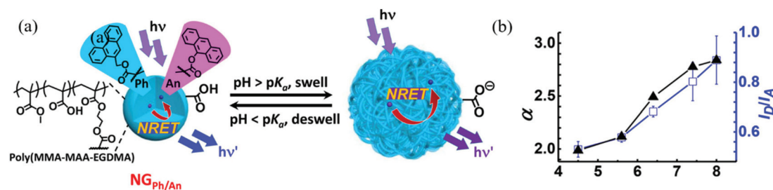
Fig. 3 (a) Schematic depicting the sensing mechanism of pH-responsive nanogel probes (NGPh/An). (b) Variation of the average linear swelling ratio ( \alpha ) and I_{Ph}/I_{An} with pH for DX NG(NGPh/An). Reprinted (adapted) with permission from ref. 67. Copyright (2017) American Chemical Society.
