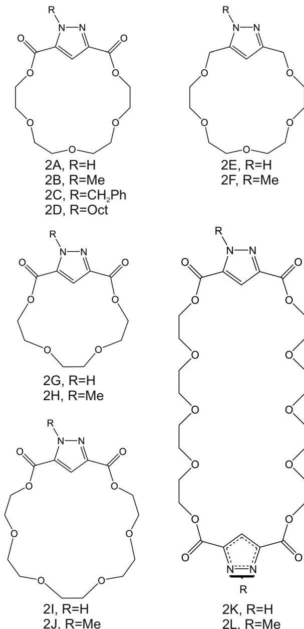
Fig. 3 Aza-crown ether derivatives, reported by Moriuchi-Kawakami et al. , as \text{NH}_4^+ ionophores. 82
