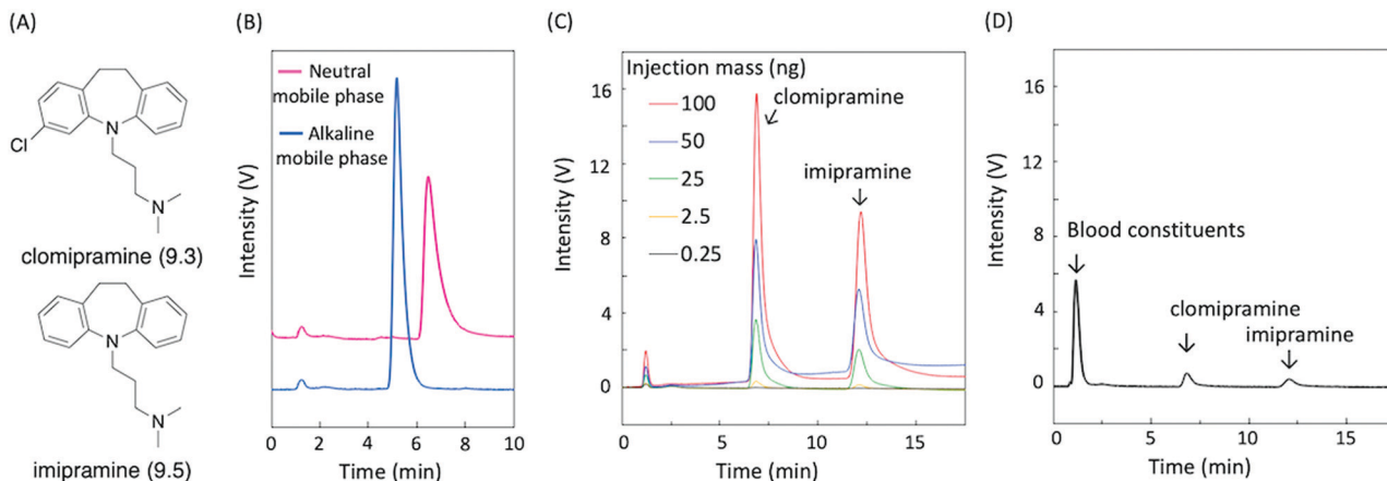
Fig. 5 (A) Chemical structures and pK_a s of the basic antidepressants clomipramine and imipramine; chromatograms of basic antidepressants for the \text{CaCO}_3\text{-PMACo} column flowed at 0.3 \text{ mL min}^{-1} . (B) clomipramine ( 0.1 \text{ mg mL}^{-1} ) with neutral and alkaline mobile phases. Methanol/water (63/37, v/v) was used as a neutral mobile phase and methanol/pH 10.8 \text{Na}_2\text{B}_4\text{O}_7 buffer (63/37, v/v) was used as an alkaline mobile phase. (C) Mixture of two basic antidepressants (clomipramine and imipramine) with a methanol/pH 10.8 \text{Na}_2\text{B}_4\text{O}_7 buffer (55/45, v/v). (D) Basic antidepressants (clomipramine and imipramine) spiked into whole blood of porcine with a methanol/pH 10.8 \text{Na}_2\text{B}_4\text{O}_7 buffer (55/45, v/v).
