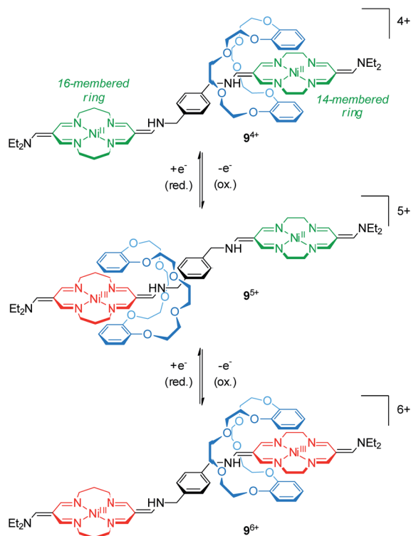
Fig. 9 Redox-controlled molecular shuttle 9^{4+} based on the cyclodene/crown ether motif in its three stable oxidation states ( \text{Ni}^{\text{II}}/\text{Ni}^{\text{I}} , \text{Ni}^{\text{III}}/\text{Ni}^{\text{II}} and \text{Ni}^{\text{III}}/\text{Ni}^{\text{III}} ).
