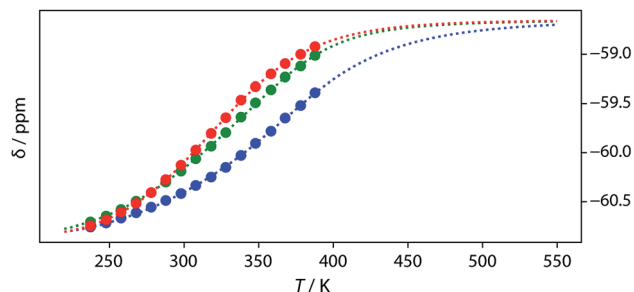
Fig. 11 ^{19}\text{F} NMR (500 MHz, TCE- \text{d}_2 , 7.4 mM) melting experiments. The lines show fitting of a two-state equilibrium isochore to the AD data (red) and a three-state isochore to the ADAD data (inner residue green, outer residue blue).
