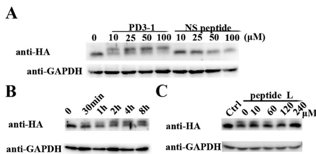
Fig. 4 The covalent reaction in HA-PDZ ARG53 transfected cell lysates. (A) Covalent bonding of peptide PD3-1 or peptide NS to HA-PDZ ARG53 after 8 h incubation at room temperature with HA-PDZ ARG53 transfected cell lysates. (B) Reaction kinetics study of peptide PD3-1 and HA-PDZ ARG53 conjugation in HA-PDZ ARG53 transfected cell lysates for 0 min, 30 min, 1 h, 2 h, 4 h and 8 h respectively. (C) The high concentration of linear peptide competitively blocked the labeling of peptide PD3-1 (30 μM) to HA-PDZ ARG53 in cell lysates in a dose-dependent manner.
