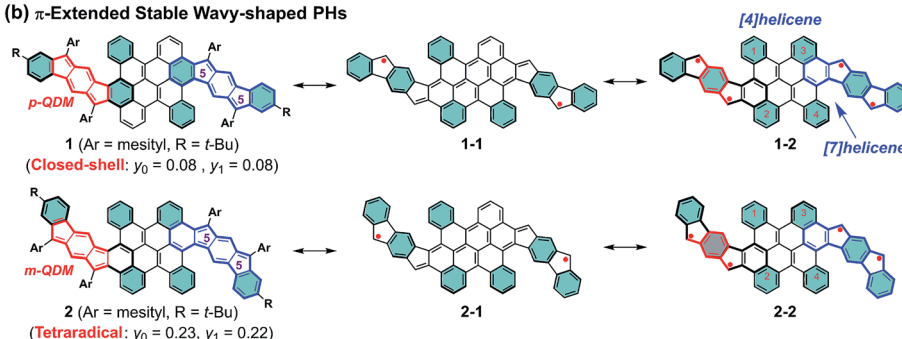
Fig. 1 (a) Representative curved \pi -systems. (b) The resonance structures of \pi -extended stable wave-shaped PHs 1 and 2 reported in this work ( p -QDM and m -QDM units are highlighted in red color; the flanked indeno[1,2- b ]fluorene (IF1) and indeno[2,1- b ]fluorene (IF2) in 1 and 2 are highlighted in blue color). The substituents are omitted in the resonance structures for clarity and the benzene rings in cyan color denote Clar's aromatic sextet rings.
