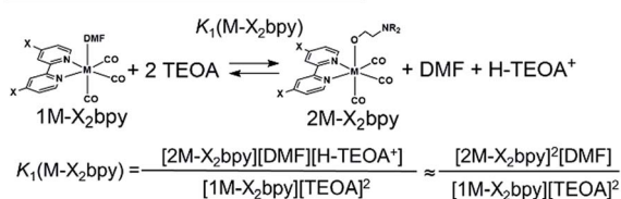
Process 1 (Ligand substitution reaction)
