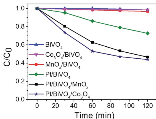
Fig. 5 Photocatalytic degradation of CBZ on different photocatalysts. Reaction conditions: 100 mL CBZ solution with initial concentration of 10 mg L -1 , catalyst dosage 1 g L -1 , the contents of the deposited Pt is 0.2 wt%, Co 3 O 4 and MnO x are all 0.1 wt% and 300 W Xe lamp ( \lambda > 420 nm), top irradiation.
