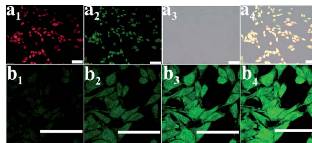
Fig. 5 Fluorescence images of HeLa cells (a) red channel indicating PCNH fluorescence ( a_1 ), green channel corresponding to DCFH-DA ( a_2 ), bright field ( a_3 ) and the merged image ( a_4 ). (b) ROS cumulative production photographs taken by a confocal laser scanning microscope with DCFH-DA as the indicator (excitation interval is 2 min).
