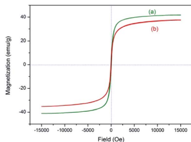
Fig. 8 VSM magnetization curve of (a) \text{Fe}_3\text{O}_4@\text{SiO}_2 and (b) \text{NH}-\text{Cu}(\text{II})@\text{MNP} .
