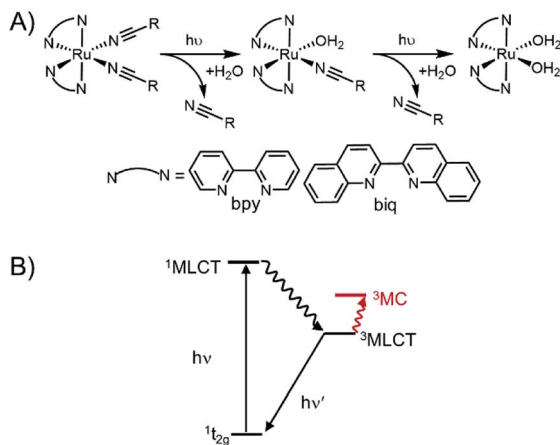
Fig. 1 Photoligated ligand exchange in ruthenium polypyridyl complexes. (A) Photolysis observed for Ru(II)-nitrile complexes is a two-step process in which both ligands are exchanged with coordinating solvent. (B) Jablonski diagram showing excited states responsible for ligand.
