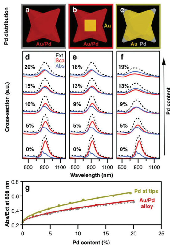
Fig. 5 Influence of Pd on the optical properties: uniform Pd distribution of Pd (a) throughout the entire particle, (b) in the branches but not in the core, and (c) only at the tips. (d–f) Corresponding extinction (black dashed), scattering (red), and absorption (blue) cross-sections, calculated by FDTD. For increasing Pd content, the scattering contributions decrease, whereas the absorbing contributions increase. Spectra are offset for clarity. (g) Pd located at the tips has a stronger effect on the absorption-to-extinction ratio, compared to octopods made of Au/Pd alloy with (red line) and without Au core (grey dashed line).
