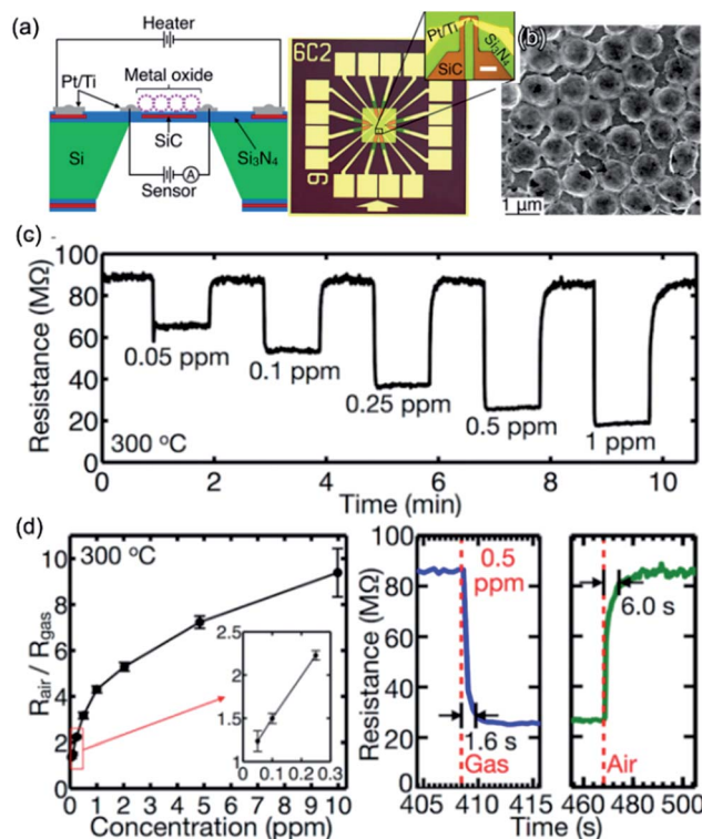
Fig. 7 (a) Schematic diagram and (b) morphology of the as-fabricated sensor with the integration of microheater platform and macroporous SnO 2 hollow spherical array. (c) Real-time sensor resistance transient to HCHO at 300 °C. (d) Sensor response versus HCHO concentration, and real-time sensor response and recovery behaviors to 0.5 ppm HCHO. Reproduced with permission. 84 Copyright 2017, American Chemical Society.
