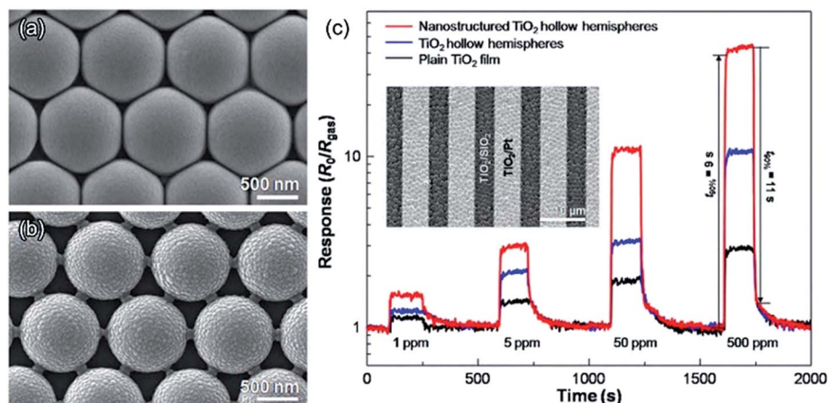
Fig. 6 Top-view SEM images of (a) TiO 2 hollow hemispheres and (b) nanostructured TiO 2 hollow hemispheres (pointy contact between hemispheres); (c) sensing transients of plain TiO 2 film, hollow hemispheres, and nanostructured hollow hemispheres to 1–500 ppm CO at 250 °C. Reprinted with permission. 82 Copyright 2010, Elsevier Ltd.
