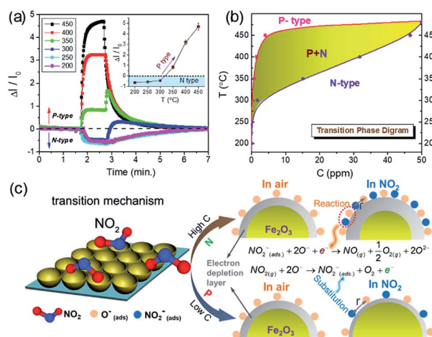
Fig. 8 (a) NO 2 response of 2DOM Fe 2 O 3 at different temperatures ( T ) and concentrations ( C ). (b) T – C transition phase diagram. (c) Schematic illustration of different NO 2 sensing types at high and low C values, respectively. Reproduced with permission. 98 Copyright 2015, Royal Society of Chemistry.
