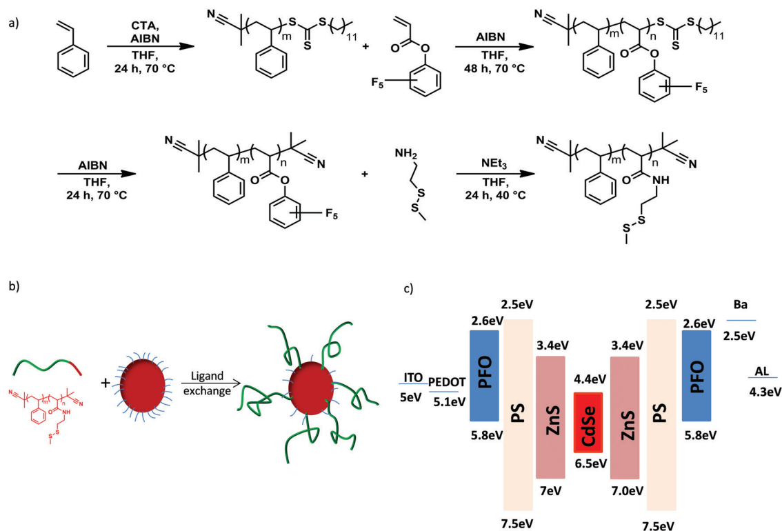
Fig. 2 (a) Synthesis of diblock copolymer poly(styrene- block -cysteaminemethylidysulfide) (P(S- b -SSMe)), (b) the ligand exchange procedure and (c) energy-band diagram of PFO:QD system.
