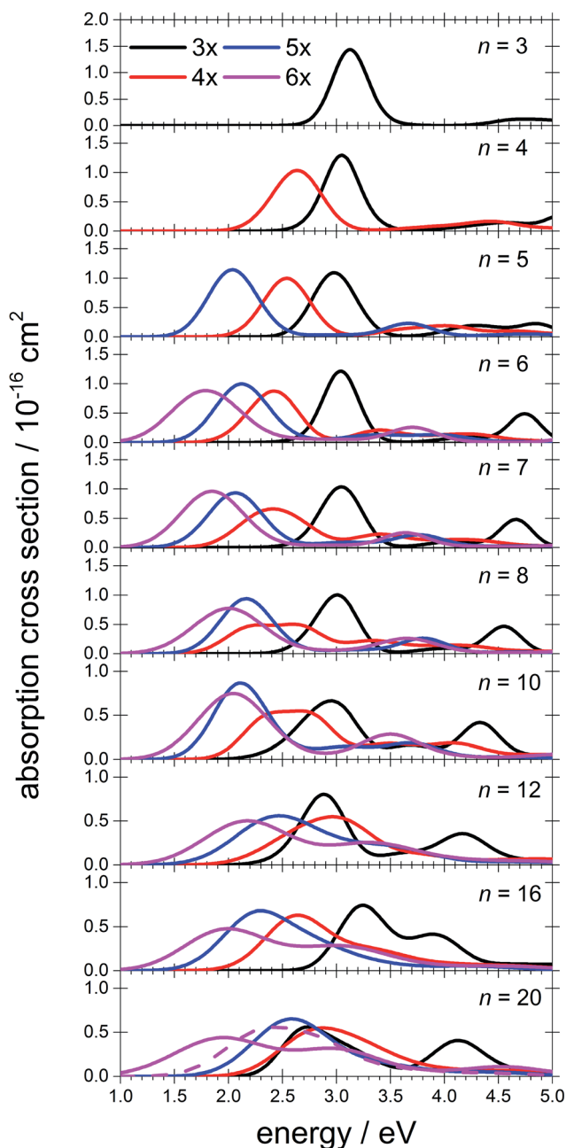
Fig. 2 Calculated spectra of selected [\text{Mg}(\text{H}_2\text{O})_n]^+ ions with different Mg coordination numbers ( 3\times-6\times ). Calculated at the CAM-B3LYP/aug-cc-pVDZ// \omega B97XD/def2TZVP level of theory using the linearized reflection principle to calculate the peak width. Surface and inner isomers for n = 20 are shown with full and dashed lines, respectively. Benchmarking with respect to the ADC(2) method can be found in Fig. S4.†
