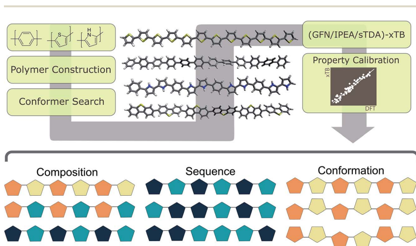
Fig. 2 Schematic of overall high-throughput approach. Starting from 2D representations of monomers (SMILES), 3D polymer models are constructed and undergo a stochastic conformer search. Optoelectronic properties are calculated using the semi-empirical xTB family of methods, which are calibrated to DFT results using a previously-determined linear model. The resulting high-throughput method is used in this work to sample compositional, sequence and conformational degrees of freedom within organic co-polymers (shown schematically using coloured pentagons, bottom).
