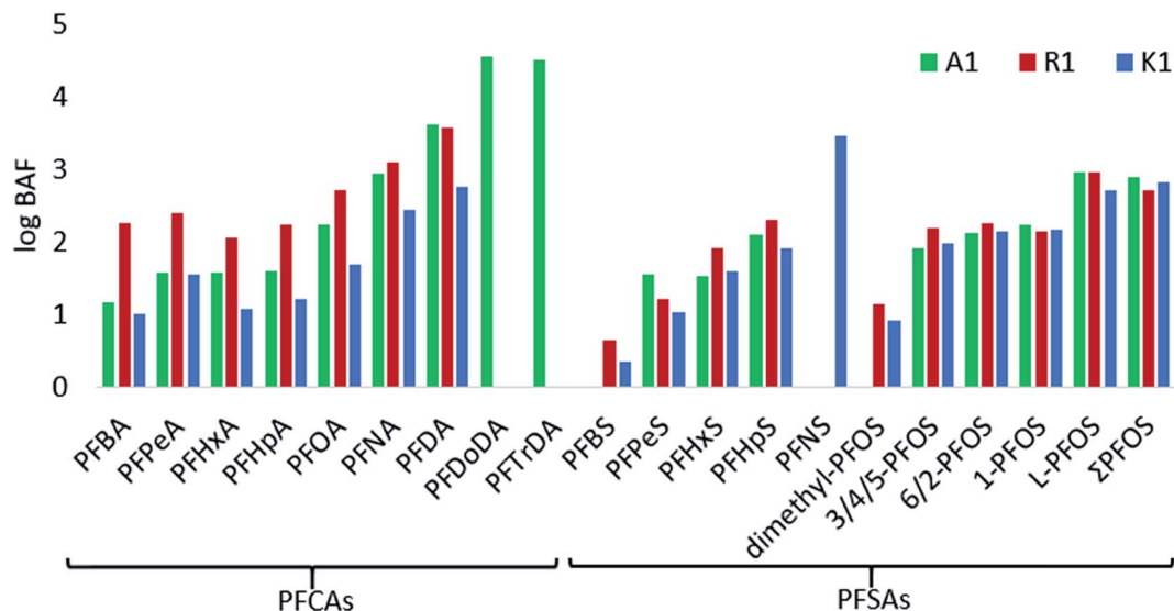
Fig. 4 The logarithmic bioaccumulation factor (BAF) on a wet weight basis ( L\ kg^{-1} ) of target PFCAs and PFSA s (including four branched PFOS isomers, linear PFOS and \Sigma PFOS) for sites A1, R1 and K1. The BAFs could not be determined for some PFSA s and sites due to values below MDL.
