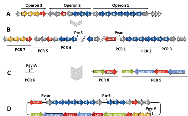
Fig. 3 BGC activation and heterologous expression strategy for the pcy biosynthetic gene cluster. (A) The native gene cluster in An d48 and its operon structure, (B) the gene cluster activated by two promoter exchanges, (C) the TAR cloning strategy including PCR pieces necessary to complete the pCIY vector and (D) the assembled heterologous expression plasmid. PKS type-II biosynthesis genes depicted in blue, regulation and resistance genes in red, exporter genes in orange, auxiliary genes for the cloning strategy in light green and ORFs of unknown function in grey colour.
