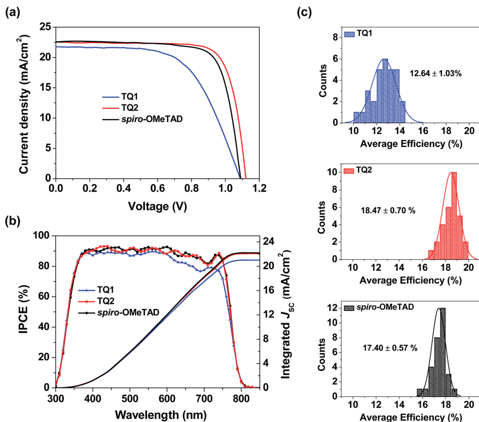
Fig. 4 (a) The J-V curves for the best-performing devices using TQ1, TQ2, and spiro-OMeTAD as HTMs. (b) IPCE spectra of the solar cell devices based on different HTMs. (c) Statistical distribution in efficiencies of the perovskite solar cells fabricated with TQ1, TQ2, and spiro-OMeTAD as the HTM, respectively.
