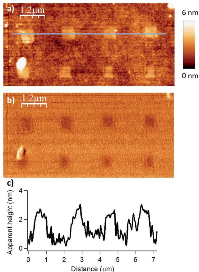
Fig. 3 Influence of the scanning speed ( V_{scan} ) on the esterification reaction with myristic anhydride as acylating reagent ( F = 2900 \text{ nN} , D_{IL} = 8 nm). The scanning speed was gradually increased from left to right with respective values of 0.25, 0.5, 1.0 and 1.5 \mu\text{m s}^{-1} for the upper line and 2.5, 5.0, 7.5 and 10.0 \mu\text{m s}^{-1} for the lower line of nanostructures. (a) Topography image in tapping mode after reaction. (b) Corresponding phase image. (c) Line profile (corresponding to the blue line in (a)) displaying an average height of 1.8 nm (theoretical calculated value of 1.78 nm in gas phase for a model, see Fig. S6 in the ESI†).
