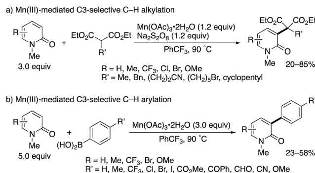
Scheme 3 \text{Mn(III)} -Mediated radical C3-selective alkylation and arylation of 2-pyridones with malonate esters and arylboronic acids, respectively.
