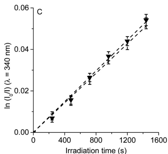
Fig. 7 First-order plots for the photooxidation of Trp (20 \mu\text{M} ) photosensitized by (A) TCP (■) and TCP in presence of D-mannitol (□), (B) TCP- \text{C}_{60} (▲) and TCP- \text{C}_{60} in presence of D-mannitol ( \Delta ) and (C) TCP- \text{C}_{60}^{4+} (▼) and TCP- \text{C}_{60}^{4+} in presence of D-mannitol ( \nabla ) in DMF/5% water; \lambda_{\text{irr}} = 562 \text{ nm} .
