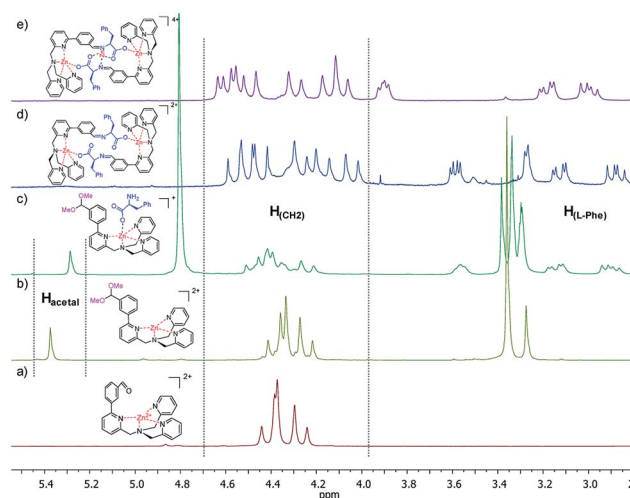
Fig. 2 Comparison of the 1 H-NMR signals for the compounds 1 , 4 , 5-L-Phe , 1-L-Phe and 2-L-Phe in D 3 -acetonitrile. In this region acetal (5.4 to 5.2 ppm), CH 2 picolyl (4.6 to 3.9 ppm) and amino acid (3.8 to 2.7 ppm) proton signals are present. The counteranions are perchlorate.
