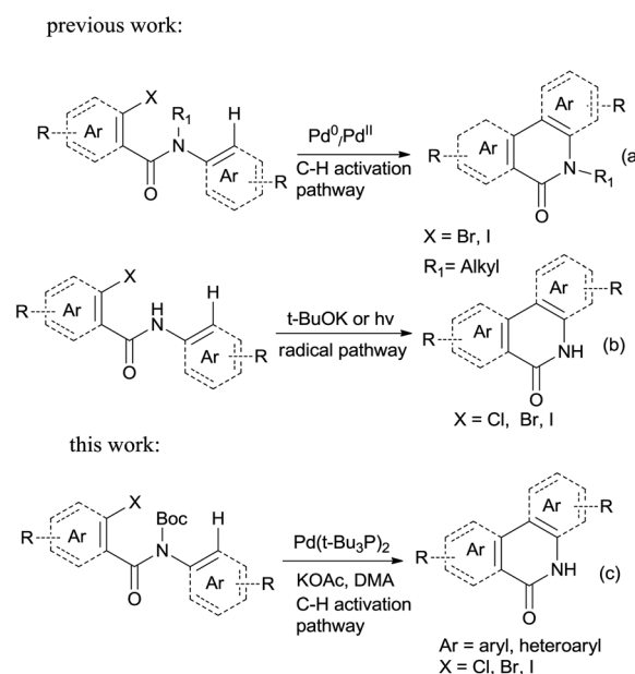
Scheme 1 Synthesis of phenanthridinones via intramolecular cyclization.
