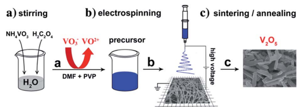
Fig. 3 Electrospinning reaction process for V_2O_5 micro/nanorods. 54
