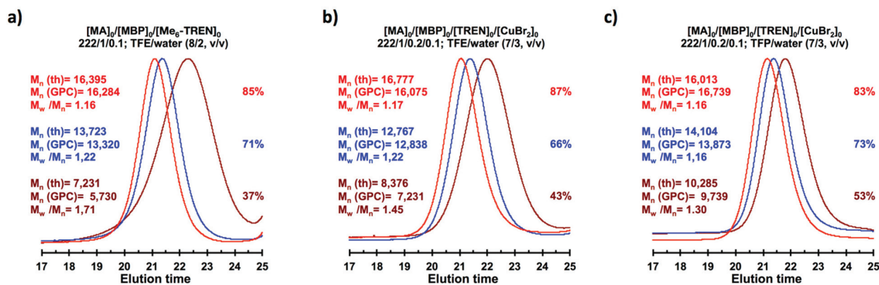
Fig. 6 GPC traces of PMA obtained by SET-LRP of MA initiated with MBP and catalyzed by nonactivated Cu(0) wire at 25 °C in (a) TFE/water (8/2, v/v); (b) TFE/water (7/3, v/v) and (c) TFP/water (7/3, v/v). Reaction conditions: (a) MA = 1 mL, TFE + water = 0.5 mL, [MA]_0/[MBP]_0/[Me_6-TREN]_0 = 222/1/0.1 and (b and c) [MA]_0/[MBP]_0/[TREN]_0/[CuBr_2]_0 = 222/1/0.2/0.1 .
