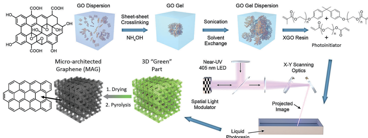
Fig. 2 Scheme of resin synthesis. GO is first crosslinked (XGO) into a hydrogel monolith then dispersed by sonication into a gel fragment dispersion. The addition of acrylates and photoinitiator creates the "XGO resin" and allows PuSL 3D printing, followed by drying and pyrolysis to the final micro-architected graphene (MAG).
