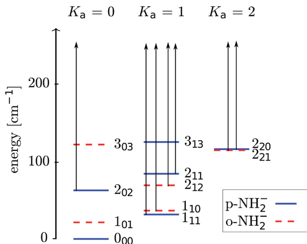
Fig. 3 Pictorial presentation of the lower rotational levels of \text{NH}_2^- ( 1A_1 ). Both ortho and para levels are shown. The arrows indicate the levels involved in the laser photodetachment process. The energy levels are labeled as J_{K_a K_c} ; in the text we use J_{\tau=K_a-K_c} notation.
