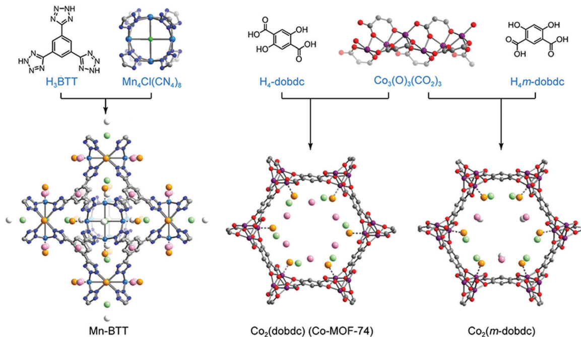
Fig. 7 (top) Molecular structures of organic linkers and inorganic building units comprising the Mn-BTT, Co 2 (dobdc), and Co 2 (m-dobdc) MOFs. (bottom) Crystal structures of each framework loaded with D 2 (16 molecules per Mn 4 Cl unit in Mn-BTT and 2.25 D 2 per Co 2+ for Co 2 (dobdc) and Co 2 (m-dobdc)). Gray, red, dark blue, blue, and purple spheres represent C, O, N, Mn, and Co atoms, respectively. Deuterium molecules adsorbed at primary, secondary, ternary, and quaternary sites are shown in large orange, light green, pink, and white spheres, respectively. D 2 -framework interactions for the primary binding site are drawn as dotted lines. Hydrogen atoms of organic linkers are omitted to clarify. 29,140
