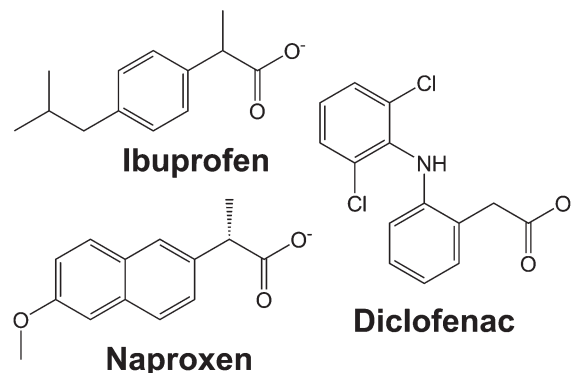
Fig. 1 The chemical structures of the anions of diclofenac, ibuprofen, and naproxen.
