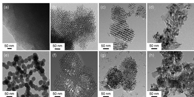
Fig. 2 TEM images of (a) the mesoporous silica template KIT-6, (b) m - \text{Co}_3\text{O}_4 , (c) m -NiO, (d) m - \text{Fe}_2\text{O}_3 , (e) Au/KIT-6, (f) Au/ m - \text{Co}_3\text{O}_4 , (g) Au/ m -NiO, and (h) Au/ m - \text{Fe}_2\text{O}_3 .
