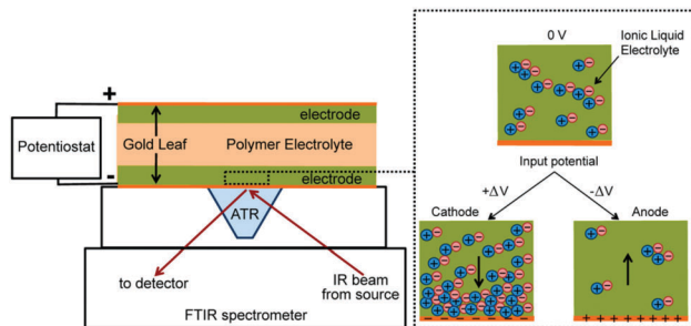
Fig. 3 In situ dynamics measurements in IPMC actuators comprising ionic liquid-embedded Nafion™ by ATR-SEIRAS. The enlarged image on the right shows ion detection at the gold/electrode interface during the measurements under a given dc voltage. Figure is adapted from ref. 60 with the permission of American Chemical Society.
