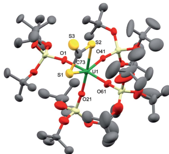
Fig. 4 Molecular structure of [U(CS 3 ){OSi(O t Bu) 3 ] 4 ] - in crystals of 7 ·tol shown with 50% probability thermal ellipsoids. [K(2.2.2-cryptand)] + , hydrogen atoms and lattice solvent have been omitted for clarity.
