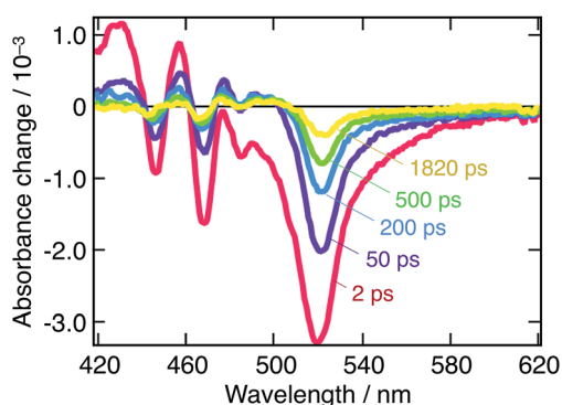
Fig. 2 Transient absorbance spectra of a suspension of \text{CH}_3\text{NH}_3\text{PbBr}_3 nanoparticles in chlorobenzene at different time delays following \lambda_{\text{ex}} = 390 nm pulsed excitation. Red: t = 2 ps, purple: t = 50 ps, blue: t = 200 ps, green: t = 500 ps, and yellow: t = 1820 ps.
