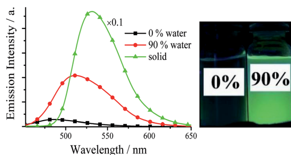
Fig. 2 Emission spectra and photographs (under 360 nm UV light) of 3,5\text{-}Cl\text{-}Cy in MeCN– H_2O with different f values ( 1.0 \times 10^{-5} \text{ mol dm}^{-3} ) and solid.
