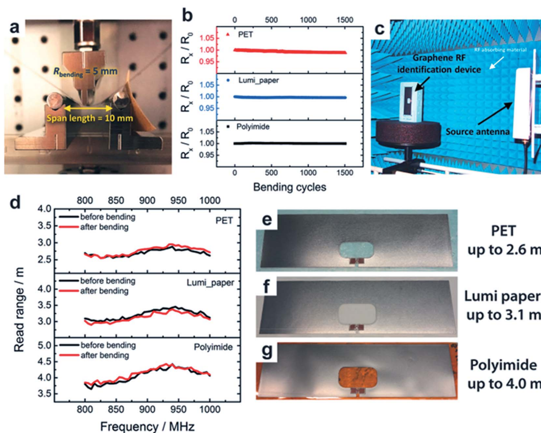
Fig. 12 Bending performance of graphene-based RFID devices. (a) Bending setup having 5 mm bending radius, 10 mm span length, and 1 Hz frequency, (b) change of resistance as a function of bending cycles up to 1500 cycles on PET, Lumi paper, and polyimide substrates, (c) graphene RFID tag measurements in an anechoic chamber, (d) frequency-dependent reading range before and after 1000 bending cycles. Photographs of graphene-based RFID devices on (e) PET, (f) Lumi paper, and (g) polyimide substrates at 867 MHz (on the right). [Reprinted with permission from ref. 192 Copyright © Wiley.]
