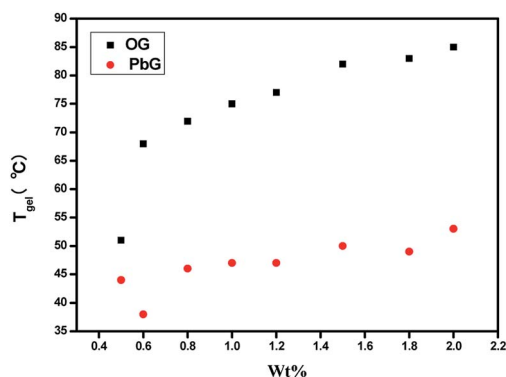
Fig. 8 Plots of T_{\text{gel}} against the concentrations of organogel OG and metallgels PbG ( G1 – \text{Pb}^{2+} = 1 : 1 ) in ethanol.
