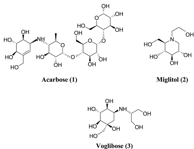
Fig. 1 Chemical structures of the well-known antidiabetics drugs.
