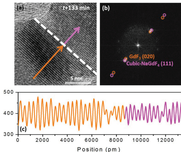
Fig. 6 (a) At t = 133 min, the HRTEM image shows a clear crystal interface between \text{GdF}_3 and \text{NaGdF}_4 indicated by a white dash line. (b) The associated FFT analysis definitely shows the co-existence of (111) of \text{NaGdF}_4 and (020) of \text{GdF}_3 with same direction. (c) Line scan indicated by the orange arrow and the pink arrow in (a) shows the averaged d -spacing for \text{GdF}_3 is 3.46 \text{ \AA} and that for \text{NaGdF}_4 is 3.17 \text{ \AA} , corresponding to the \text{GdF}_3 (020) plane and \text{NaGdF}_4 (111) plane.
