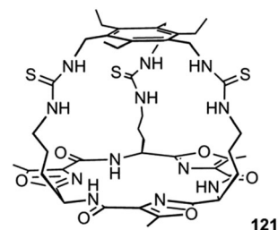
Fig. 32 The structure of compound 121 .
