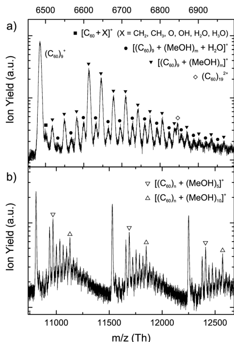
Fig. 2 (a) Expanded view of the mass spectrum for a C 60 /MeOH mixture in helium nanodroplets near the (C 60 ) 9 + peak. In addition to peaks corresponding to [(C 60 ) 9 + (MeOH) m ] + ions, we can also identify peaks from ions where one water molecule is attached to [(C 60 ) 9 + (MeOH) m ] + (circles). Also visible is the doubly ionized (C 60 ) 19 2+ ion. (b) Detail in the region of (C 60 ) 15 + – (C 60 ) 17 + . The most abundant ions are (C 60 ) n + ions, followed by mixed clusters containing both C 60 and methanol molecules. Specially abundant ions containing 5 and 10 methanol units are highlighted.
