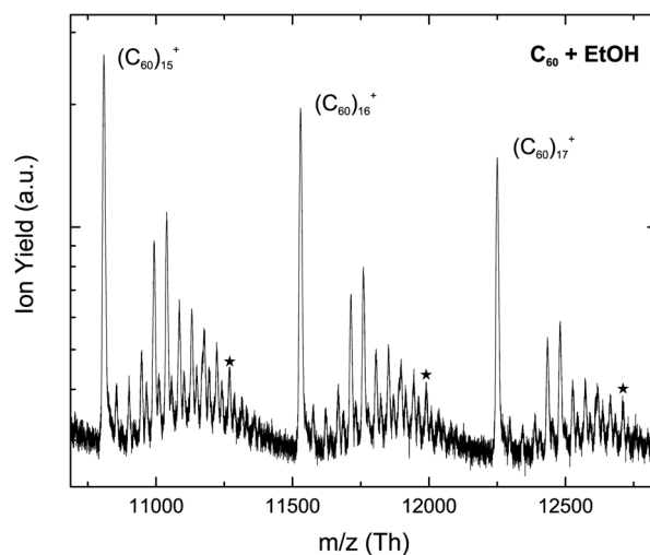
Fig. 3 A section of the mass spectrum measured upon electron ionization of helium droplets doped with C 60 and ethanol in the region of the (C 60 ) 16 + cluster. The most pronounced peaks, apart from those from bare (C 60 ) n + ions, correspond to the attachment of 4 and 5 ethanol molecules to the (C 60 ) n + cluster. The peaks labelled with an asterisk are for a (C 60 ) n + ion with 10 attached ethanol molecules.
